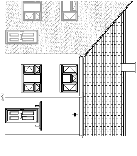
Existing Front Elevation Scale 1:100
