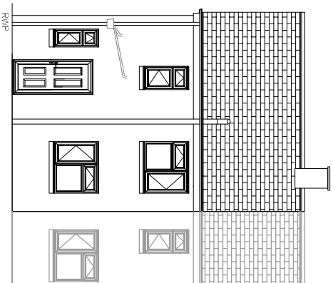
Existing Rear Elevation Scale 1:100
